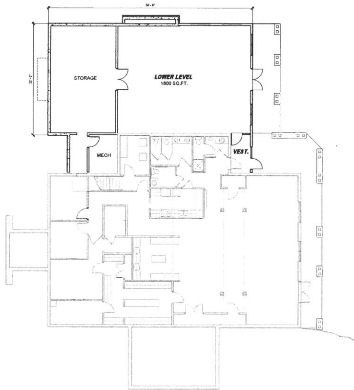
1 LOWER LEVEL 1/8" = 1'-0"
