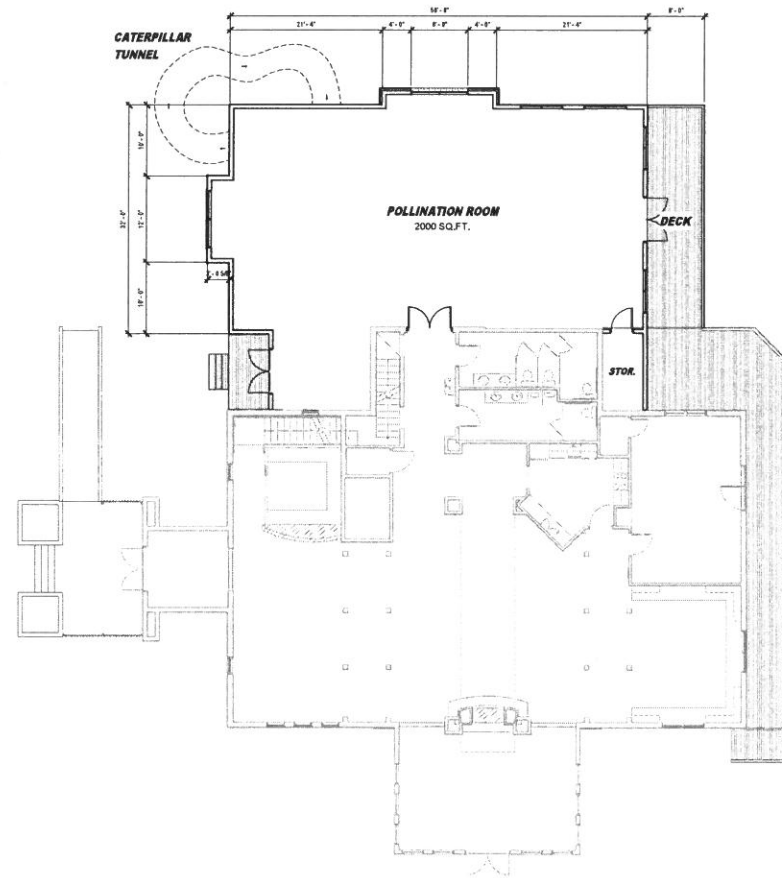
2 MAIN LEVEL 1/8" = 1'-0"
